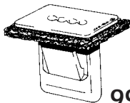
99-8238 Replaces: 25649667, W705590-S300 GROMMET - BACKGLASS MOULDINGS, DECK LID, LAMP MOUNTING, LIFTGATE & INTERIOR TRIM PANEL Plastic w/seal Hole: 9x18MM, Flange: 13x22MM, P.R.: 0.9-1.3MM, Screw: M4.2 (#8) Cadillac 'E' & 'K' Bodies '98/ & Ford Windstar '99/ UNIT PACKAGE 15
