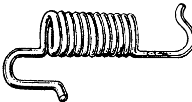
73-3820 Replaces: D4ZZ-13031A SPRING-HEADLAMP ADJUSTING Mustang, Montego Torino '74/ UNIT PACKAGE 25
