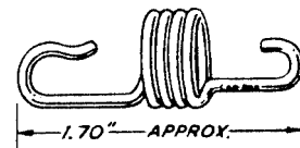
72-3649 Replaces: 1238107 SPRING-HEADLAMP ADJUSTING Buick '73 UNIT PACKAGE 25
